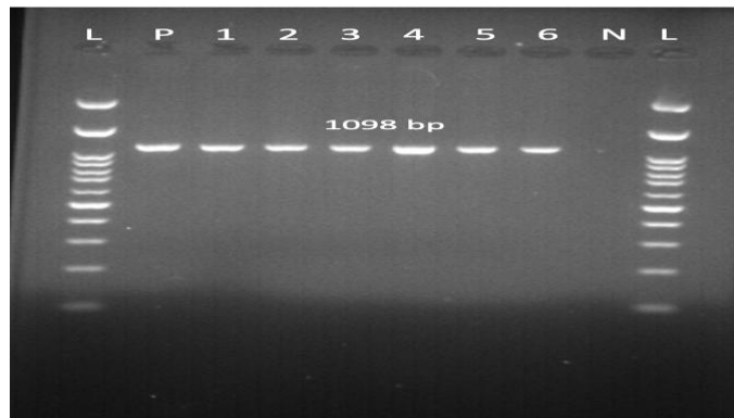
Fig. 2: PCR results of amplifying the 18S rRNA gene (1098 bp) of Theileria spp. L: 100 bp Ladder, P: Positive control, N: Negative control, 1-6 positive samples
