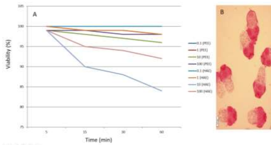
Fig. 1: A) Viability percent of E. granulosus protoscolices incubated with different concentrations of Hydroalcoholic extract (HAE) as compared with the same concentrations of petroleum ether extract (PEE). B) Dead protoscolices of E. granulosus after exposure to pumpkin seed extract with 0.1% eosin
