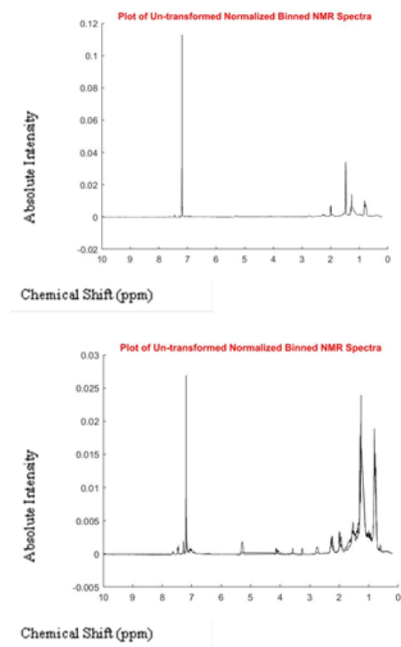
Fig. 4: Plot of Untransformed Normalized Binned NMR Spectra. (a) Control, (b) Drug test
