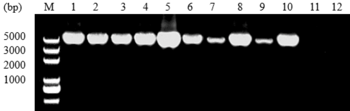
Fig. 1: Electrophoresis of PCR amplification of RON10 from different T. gondii strains M. DL5000 DNA Marker 1. RH 2. GT1 3. PYS 4. CTG 5. PRU 6. MAS 7. TgCatBr5 8. TgCatBr64 9. SH 10. TgWtdSc40 11. Host control 12. Negative control
