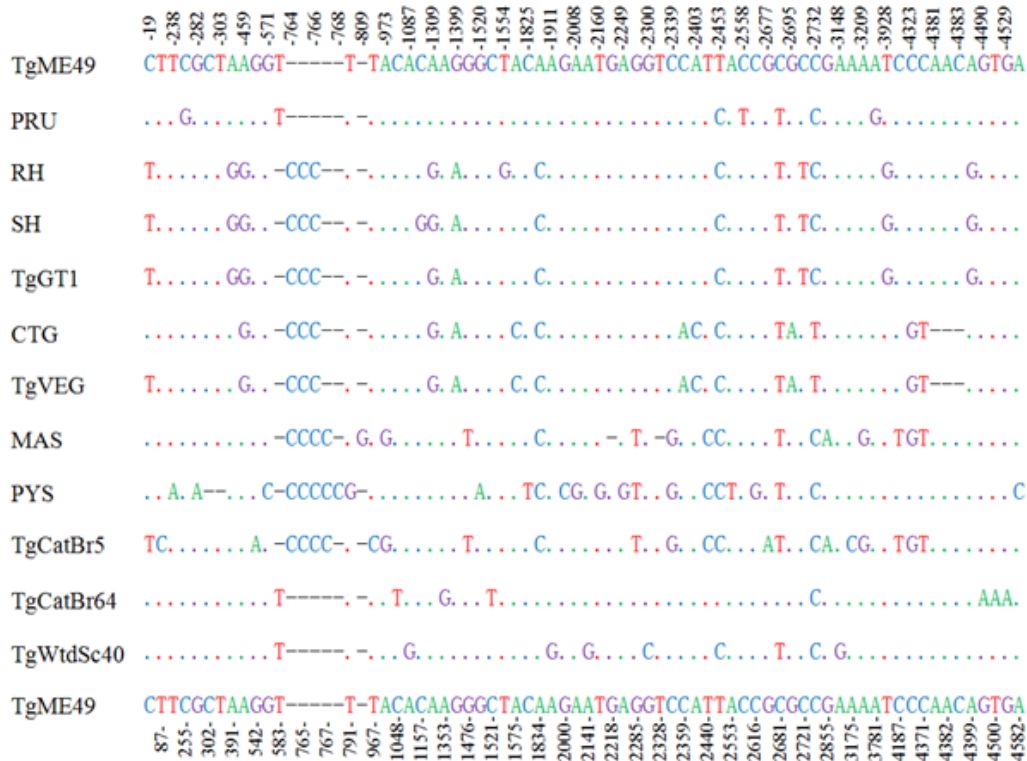
Fig. 2: Multiple alignment analyses for nucleotides sequences of Toxoplasma gondii RON10 gene Point (.) stands for identical nucleotide, dash (-) indicates nucleotide deletions in comparison to that of T. gondii ME49 strain (upper and bottom lines), and the numbers indicate the variable sequence positions for nucleotide
